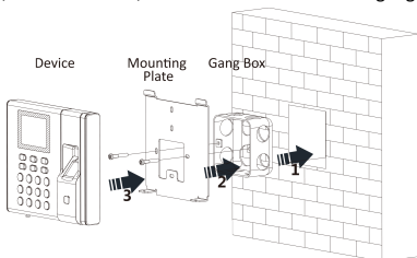
Figure 4-2 Install Device
