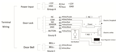
Figure 3-2 External Device Wiring
