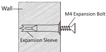
Figure 4-4 Install Expansion Screws
