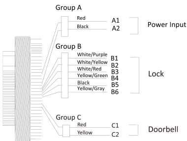
Figure 3-1 Terminal Diagram
