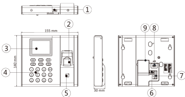
Figure 2-1 Device Appearance
