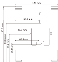
Figure 4-1 Mounting Plate
