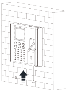
Figure 4-3 Secure Device
