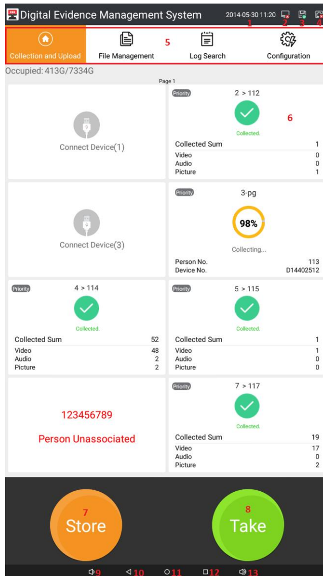
Figure 2-1 Homepage
