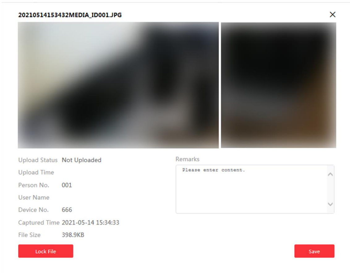
Figure 3-3 Play File
