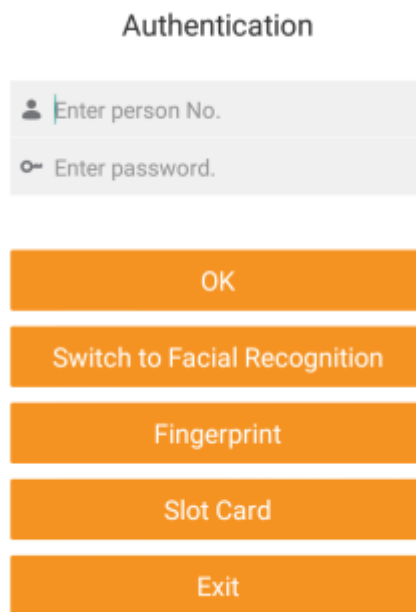
Figure 2-9 Authenticate Permission
