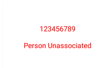
Figure 2-2 Person Unassociated
