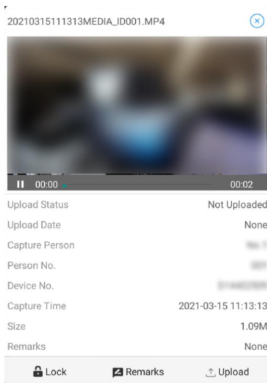
Figure 2-6 Play File
